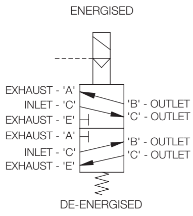
VALVE SYMBOL
